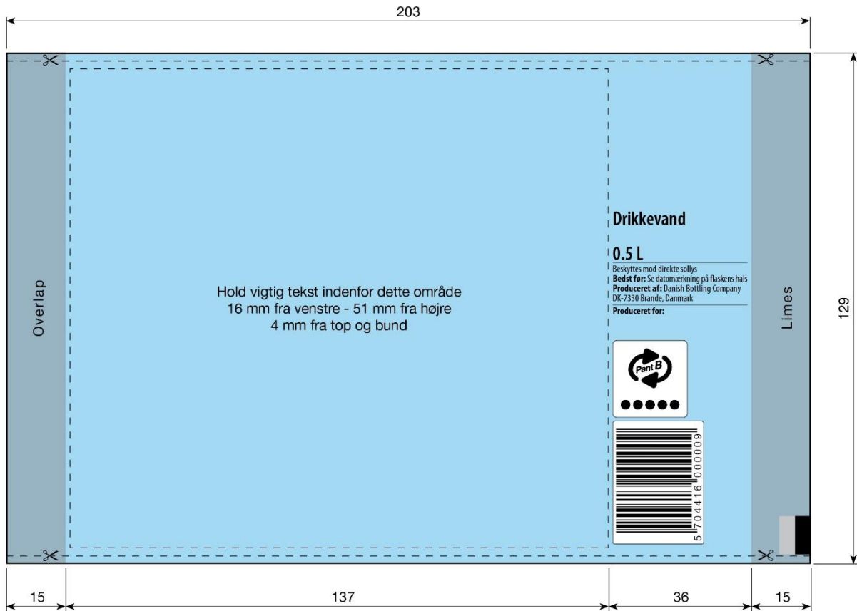
Figur: Plantegning over label – Slim 50 Plastic
